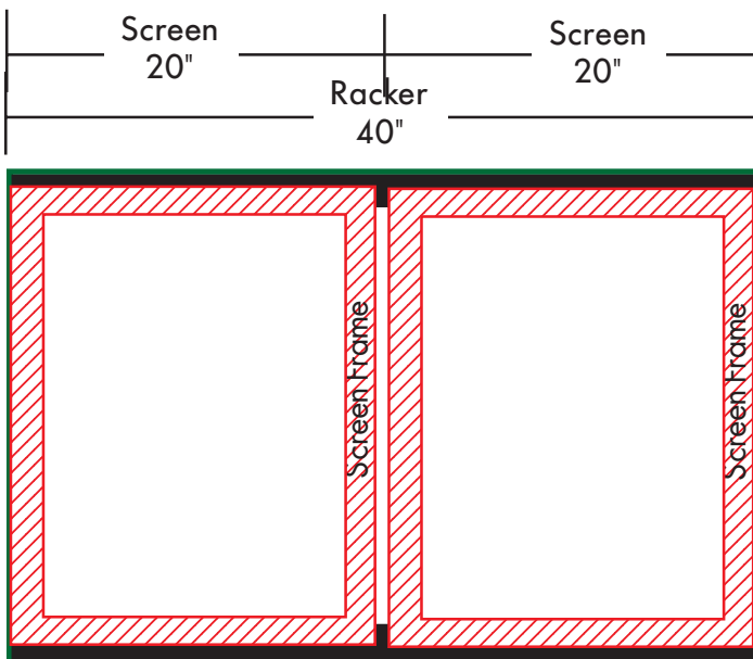
Rollin' SCREEN RACKER RSR40: 2- Screen Frames 20" x 24"
